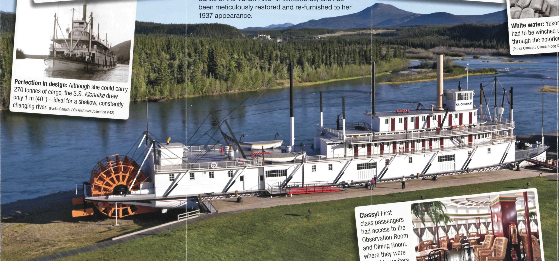
Steam Ship Klondike: Steam generated from an immense boiler powered two compound jet-condensing engines, which in turn cranked the paddle wheel. (Parks Canada / P. Gowdie)
